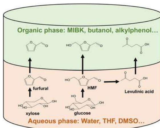
Figure 9. Organic Solvent Effects in Biomass Conversion Reactions
